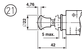
Knob – G1/8 valvole
