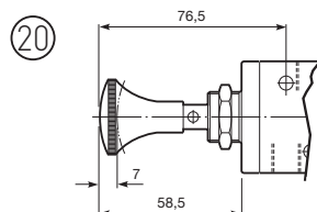
Knob – G1/4 valvole
